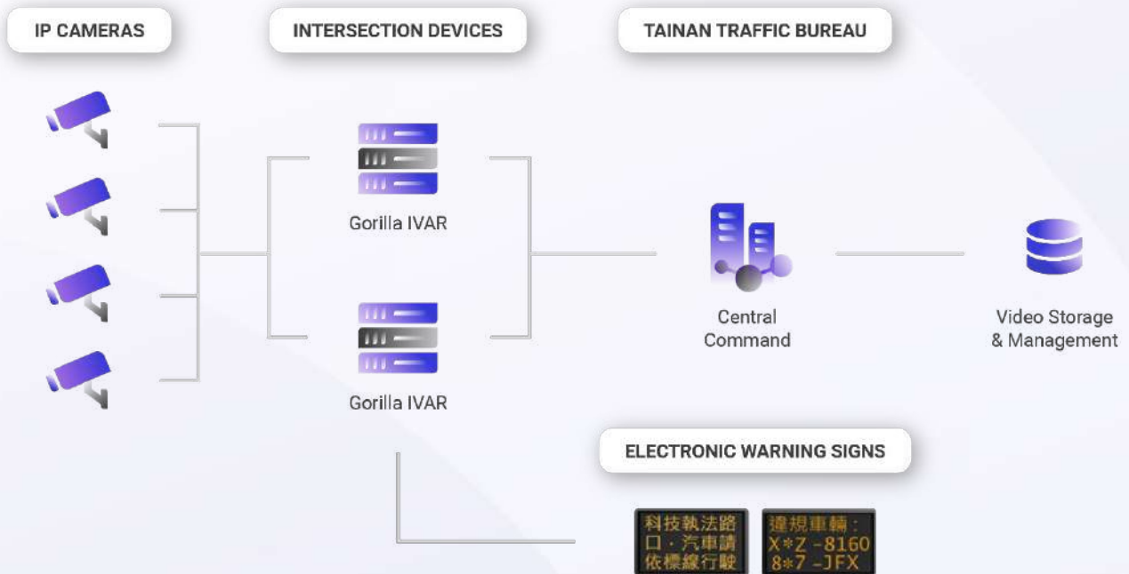
Figure 5 – Smart Intersection System Architecture
